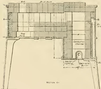
FERGUSON OIL-BURNING FLUE FURNACE.
